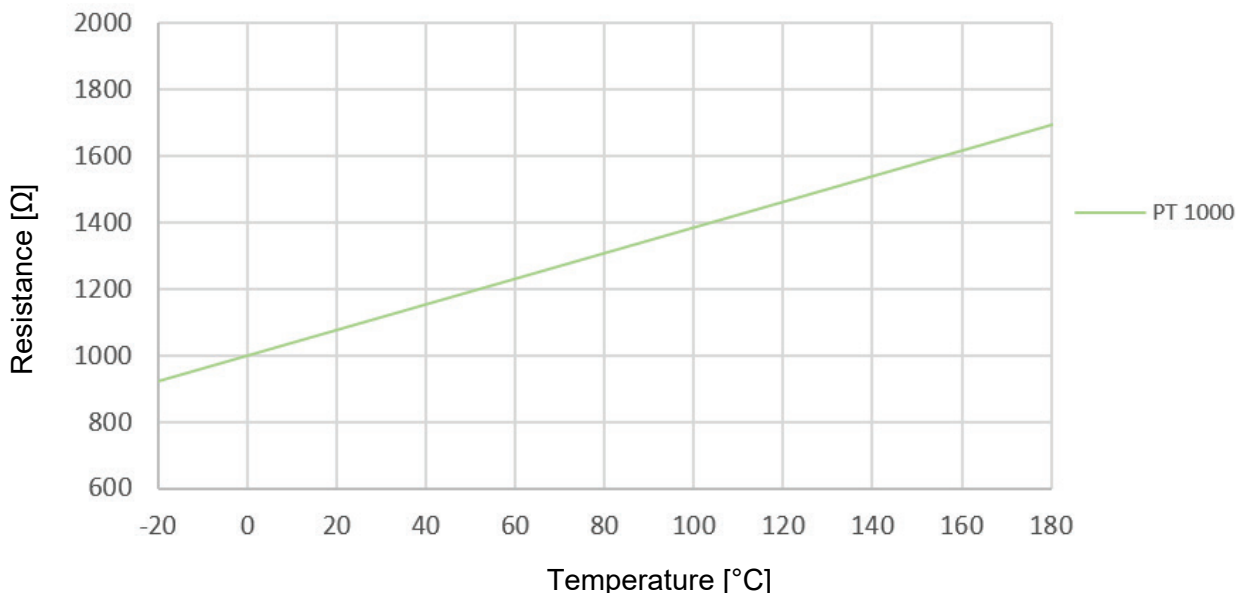
Fig. 5-6 Characteristic of the PT1000 resistance temperature chart
