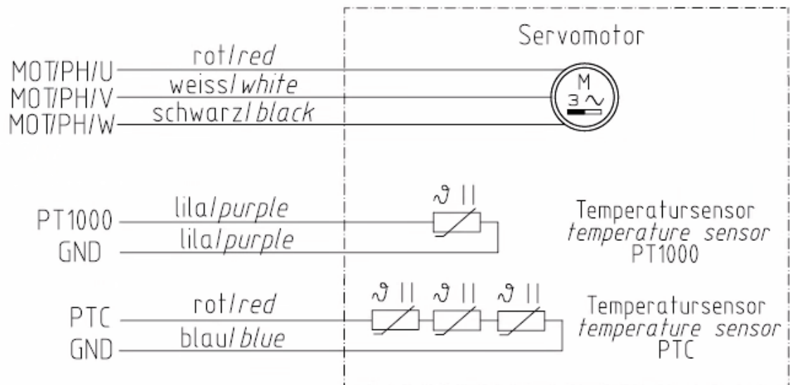
Fig. 7-1 Connection marking for power connection "A" and feedback system "NN"
