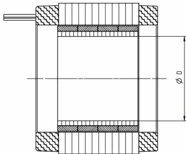
Variant 2: large inner diameter "E"
