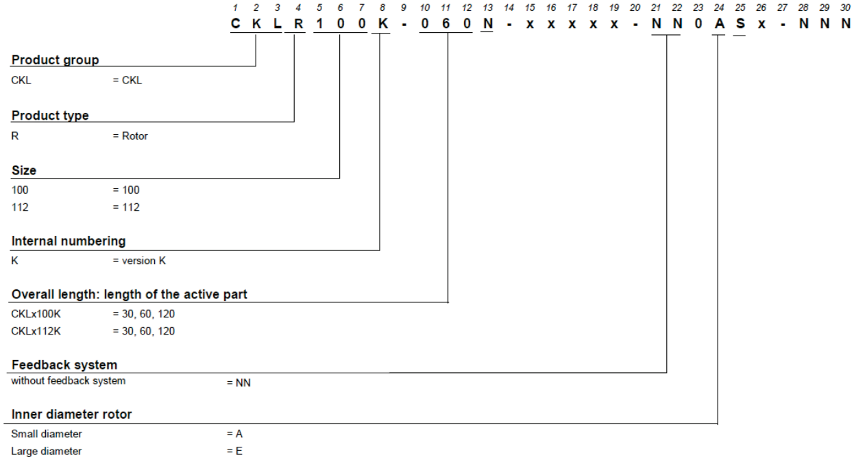
Fig. 5-4 Type code of the rotors (CKLR) of the cyber® kit line medium
