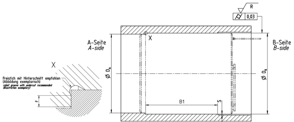
Fig. 6-2 Recommended shaft dimensions for adhesive connections
