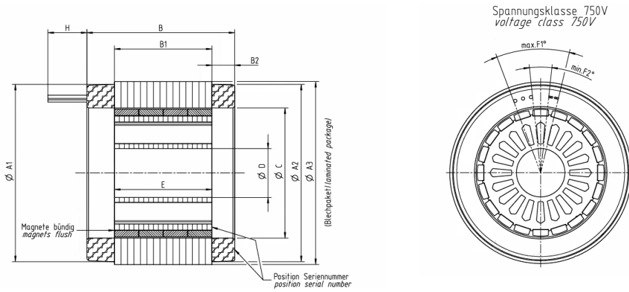
Variant 1: small rotor inner diameter "A"
