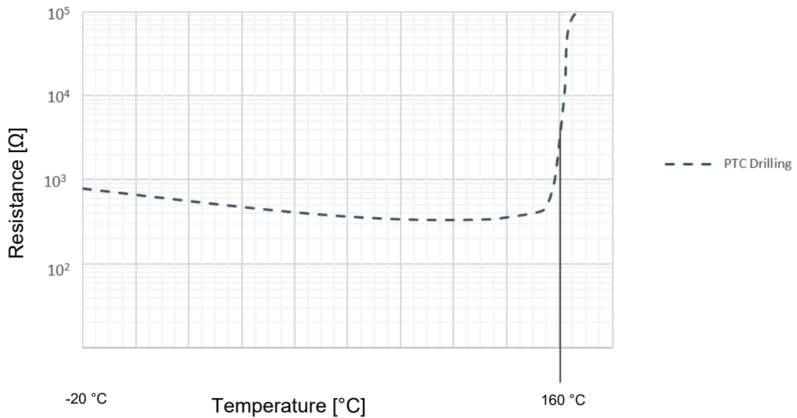
Fig. 5-7 Characteristic of the PTC twisted (type code "V"), PTC resistance temperature chart
