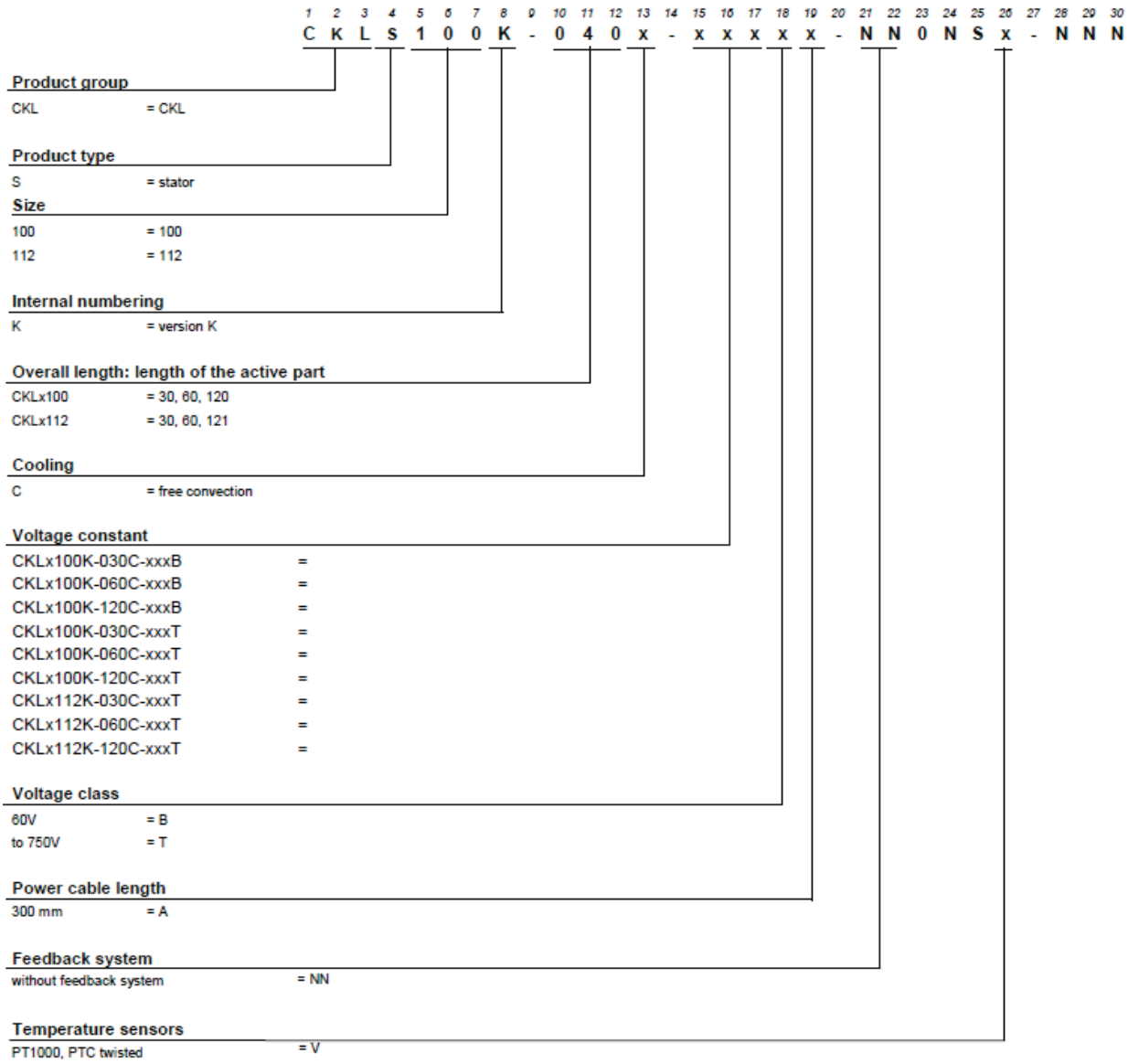
Fig. 5-3 Type code of the stators (CKLS) of the cyber® kit line medium
