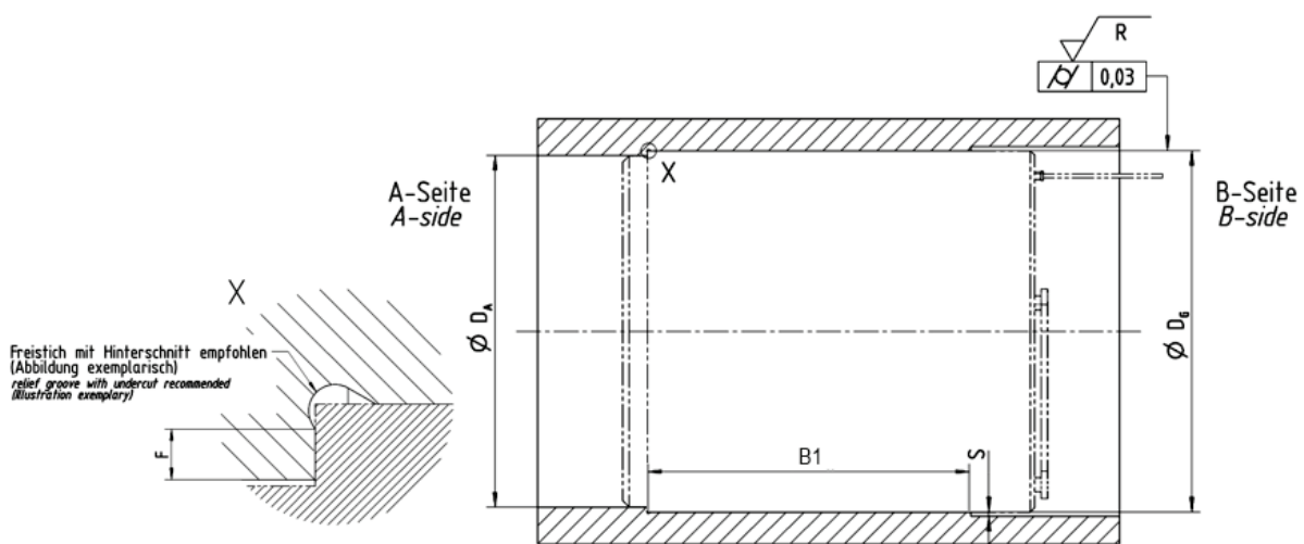
Fig. 6-1 Recommended housing dimensions for adhesive connections and clearances
