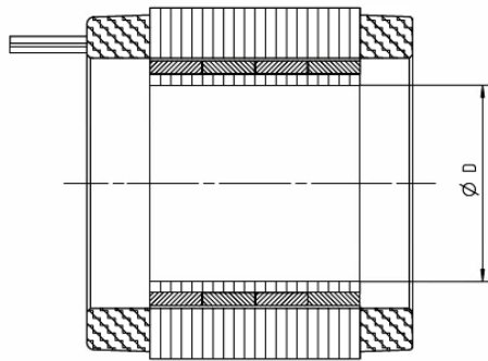
Variant 2: large inner diameter "E"
